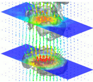
Turbulence in 3D, thanks to PIV3D and its computers
