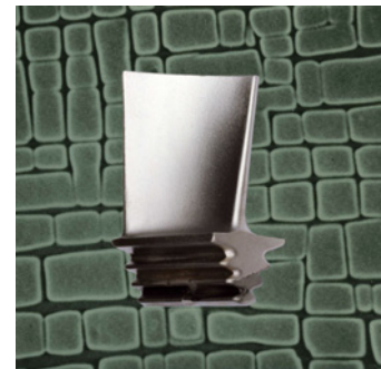
Turbine blade and microstructure of the nickel-based superalloy (AM1)
