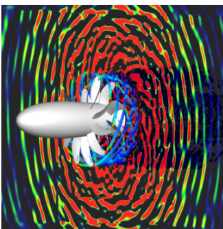
Aero-acoustic numerical simulation of a CROR double propeller
