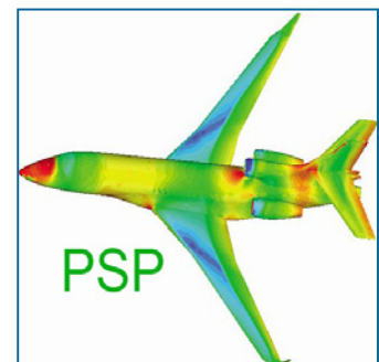
Falcon 7X model covered with pressure-sensitive paint, during a test
