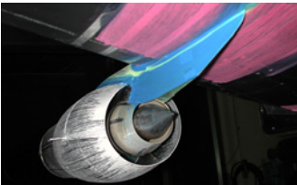
Wing-nacelle integration. Visualisation with viscous coatings (S3CH wind tunnel, Meudon)
