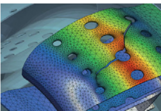
Crack propagation with ONERA's Zset Zebulon code
