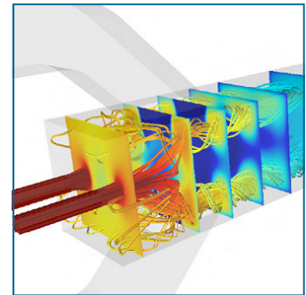
Cedre numerical simulation of combustion in an ONERA research ramjet
