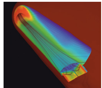
Numerical simulation of the atmospheric re-entry of the PreX demonstrator (ESA)
