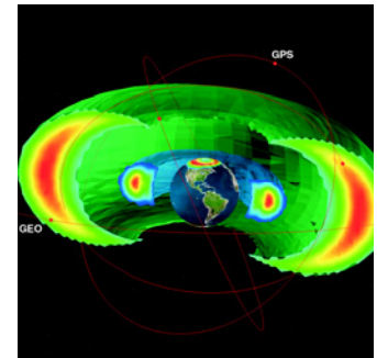
Salammbô physical model of Earth's radiation belts, a space weather tool
