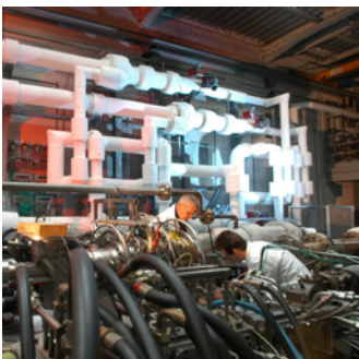
The M1 bench for studying combustion chambers (realistic conditions of cruising flight)
