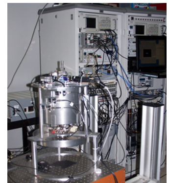
Core of the atomic interferometer in the laboratory, with its operating and measurement windows
