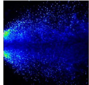
Dispersion of kerosene droplets in a combustion chamber (LIF)
