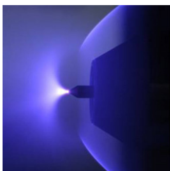
Supersonic experimentation in the R1CH gust wind tunnel on drag reduction with plasma
