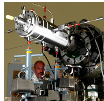
Wind-tunnel force measuring device
