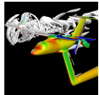
elsA numerical simulation for the European project Nicetrip
