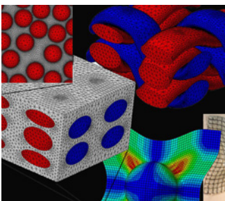
Cascading multiscale model of the behaviour and damage in 3D woven composites
