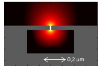
Sub-wavelength structures interacting directly with photons
