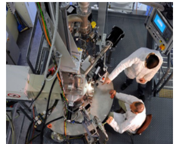
Spray tower to develop materials through powder metallurgy and to develop parts through additive manufacturing
