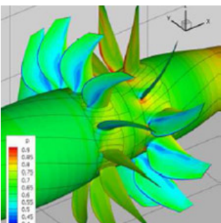
Simulation of static aeroelastic couplings on a counter rotating open rotor
