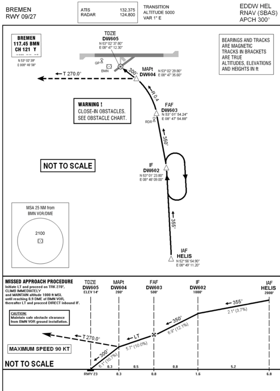
Figure 2: Helicopter specific steep and curved IFR approach procedure initially developed for Bremen airport (EDDW)
