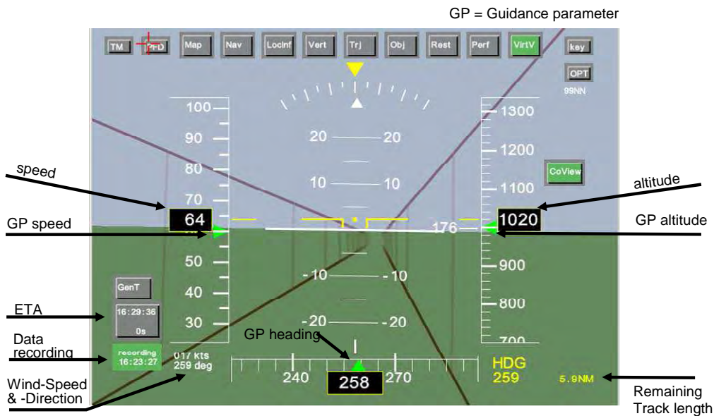
Figure 3: “Tunnel in the sky”-Display
