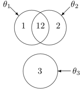
Figure 3.2: Venn Diagram for \mathcal{M}
