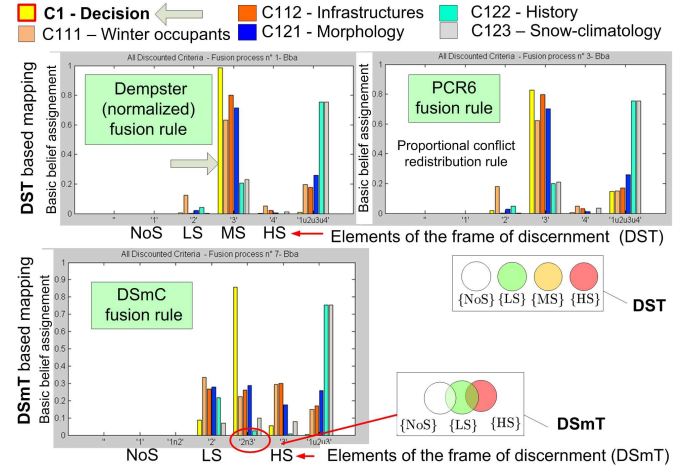
Figure 16. Comparison of fusion results.
