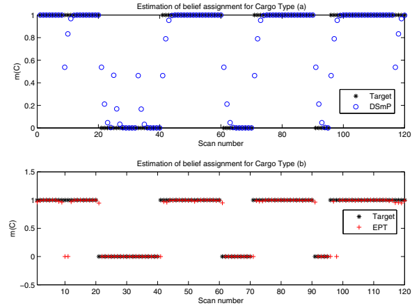
Figure 5: Belief Mass for Cargo Type for M_1 .
