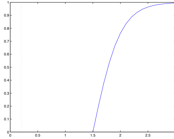
Figure 14.6: m(\theta_1 \cup \theta_2) as function of \rho given by (14.9)
