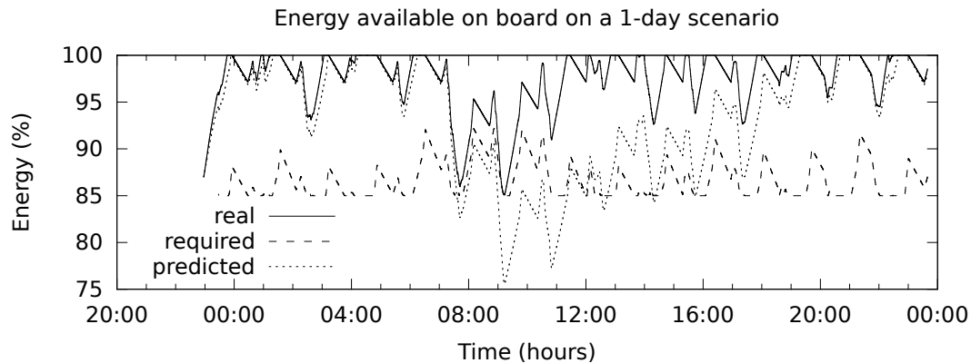
Figure 4: Satellite energy profiles (in percentage of the maximum energy level E_{max} ) over a 24-hour scenario ( E_{min} = 0.85 \cdot E_{max} ). The dotted line is the first ground prediction with margins produced by the GroundFine approach. The dashed line represents the required levels of energy computed on the ground by the Flexible approach. The solid line represents the actual energy profile resulting from the onboard execution of the Flexible approach.
